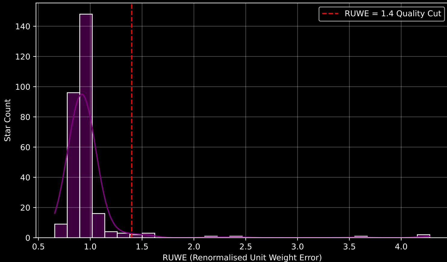
GAPOGEE DR17 Field [355-08] RUWE Distribution (n= 286)
