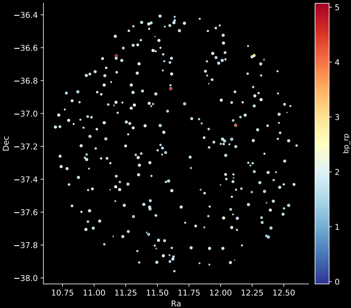
APOGEE DR17 Field: [355-08] Stars: 288
