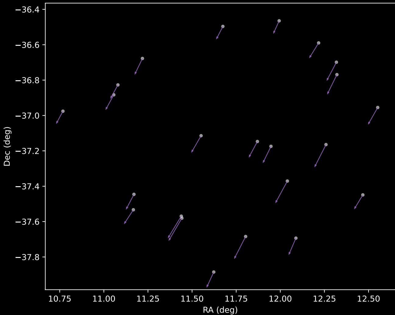
APOGEE DR17 Cluster 8 Proper Motion Vectors (n=23)
