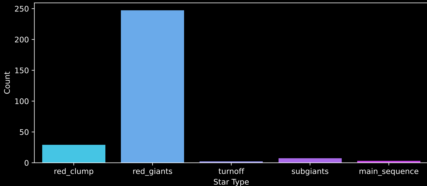
APOGEE DR17 Field: [355-08] Count plot of Star Type
