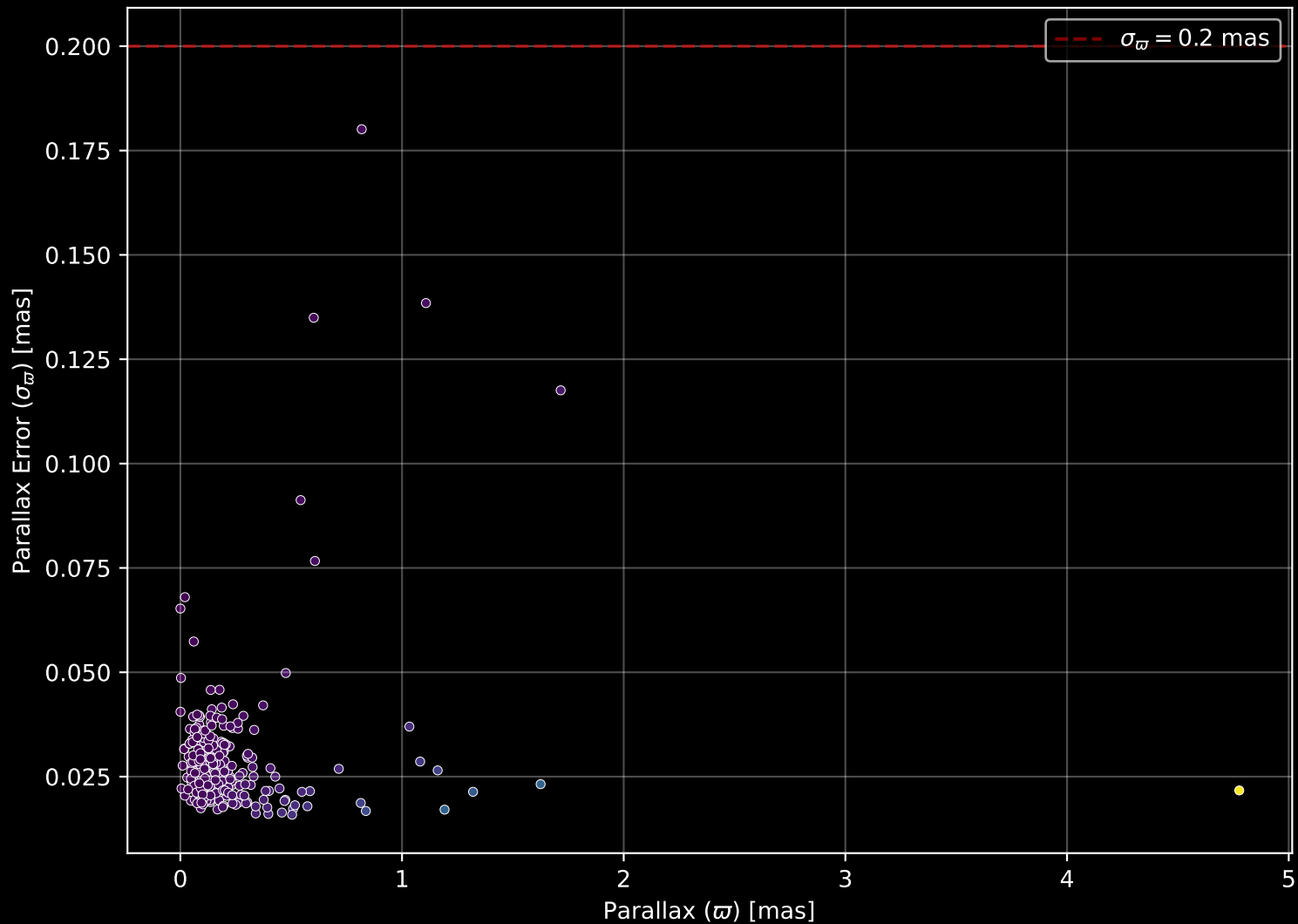
APOGEE DR17 Field: [355-08] Parallax Quality (n= 288)
