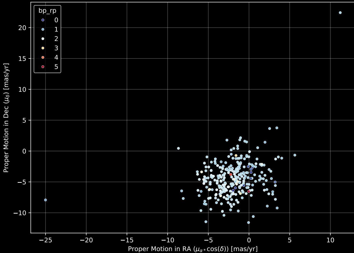
APOGEE DR17 Field: [355-08] Proper Motion Diagram (n= 288)
