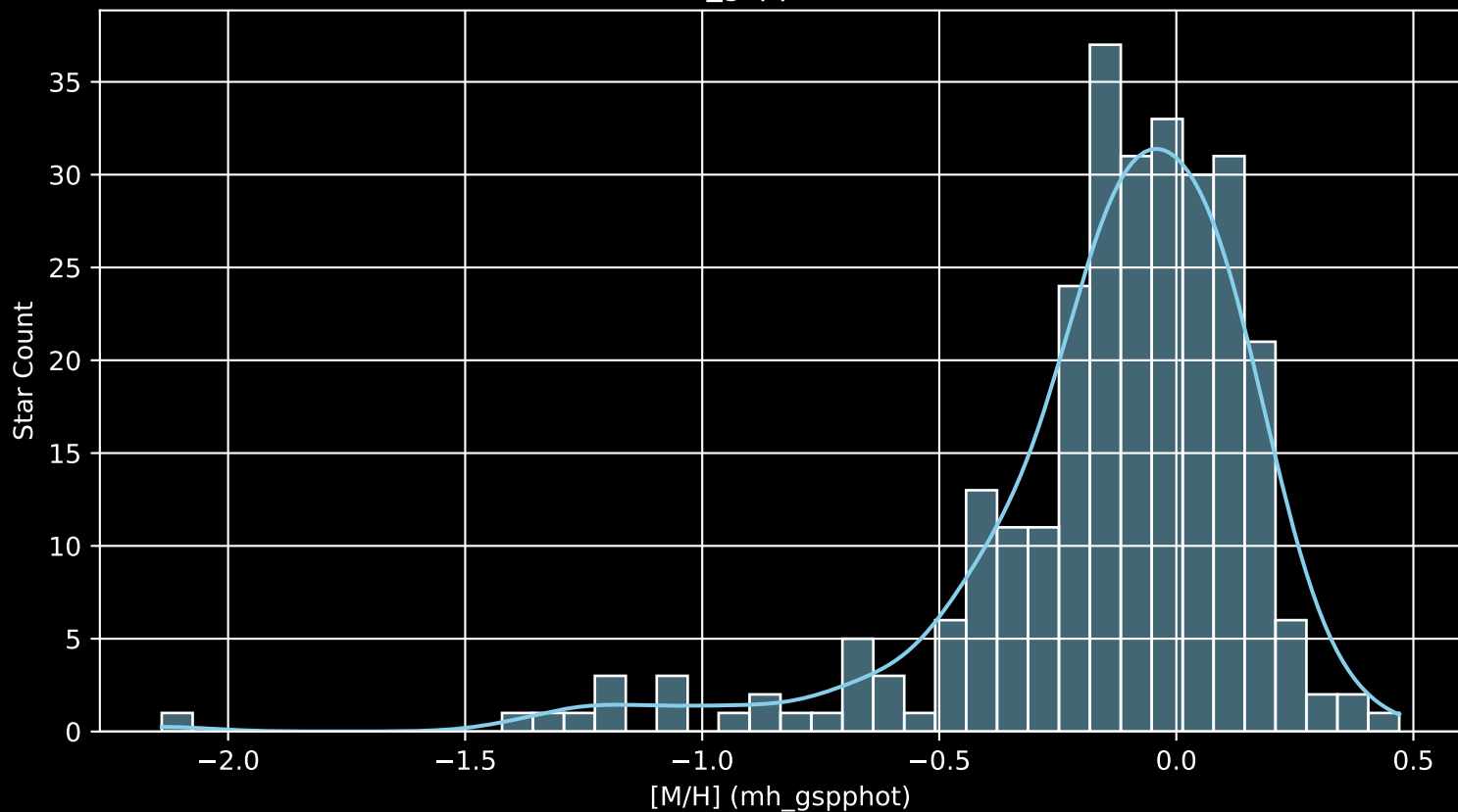
APOGEE DR17 Field: [355-08 [M/H] (mh_gspphot) (n= 283)
