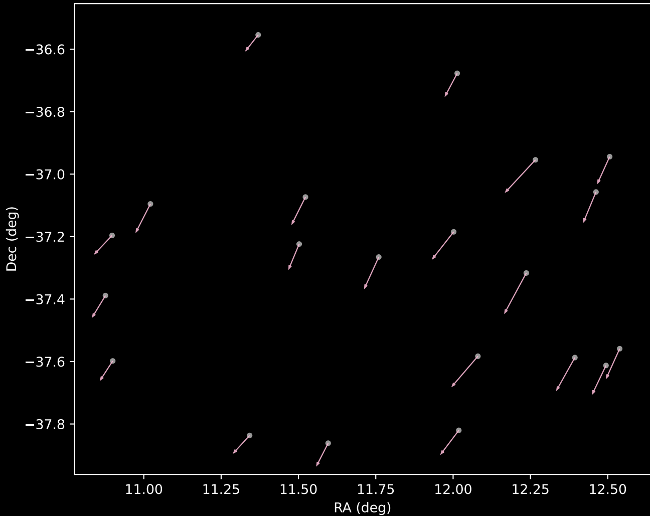
APOGEE DR17 Cluster 13 Proper Motion Vectors (n=21)
